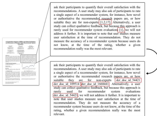
Figure 4: Converting in-text citations to Docear-IDs
