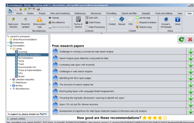
Figure 2: User-interface of Docear's recommender system
